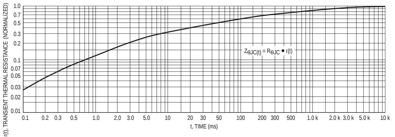
Figure 5. Thermal Response
