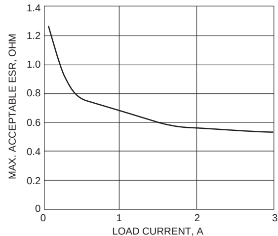
FAN1582 Stability
