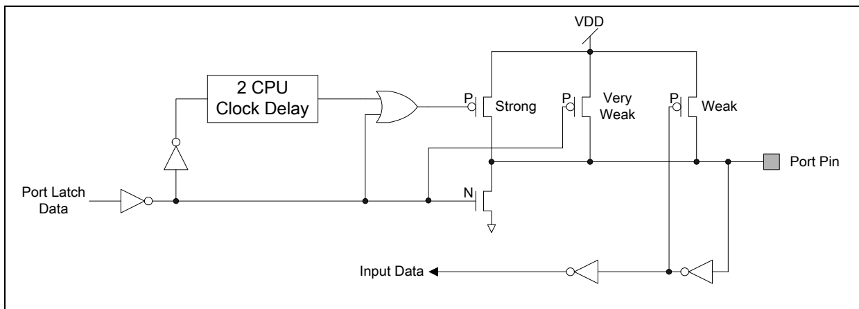
Figure 5-10 Quasi-bidirectional I/O Mode
