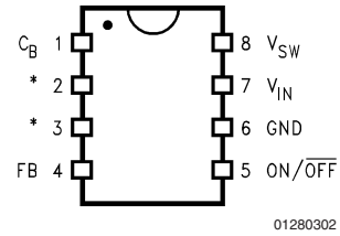
SO-8/DIP Package
