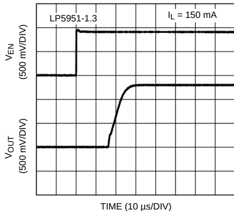
Figure 5. Enable Start-Up Time
