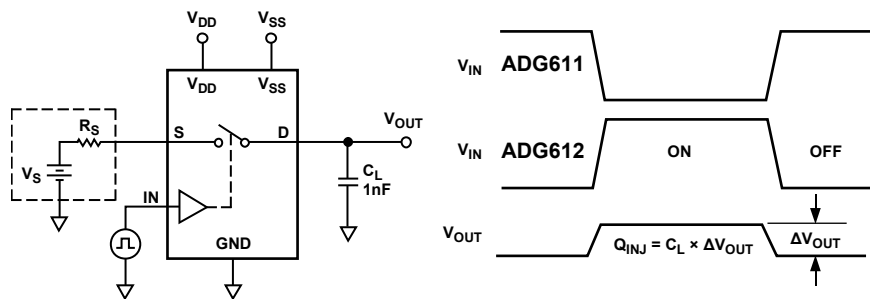
Figure 19. Charge Injection
