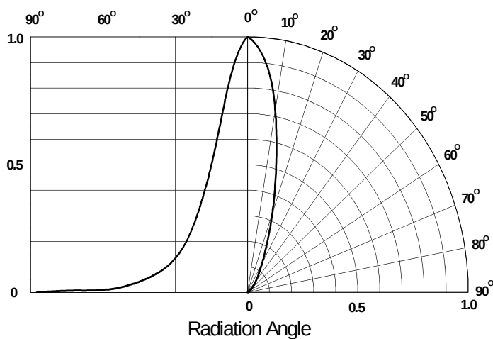
Radiation Characteristics
