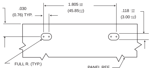
Figure 3 Edgeboard Mounting
