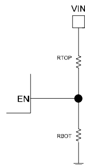
Figure 1. EN Divider Network
