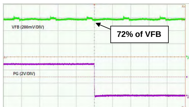
Time- 1µs/div Powergood Falling Threshold
