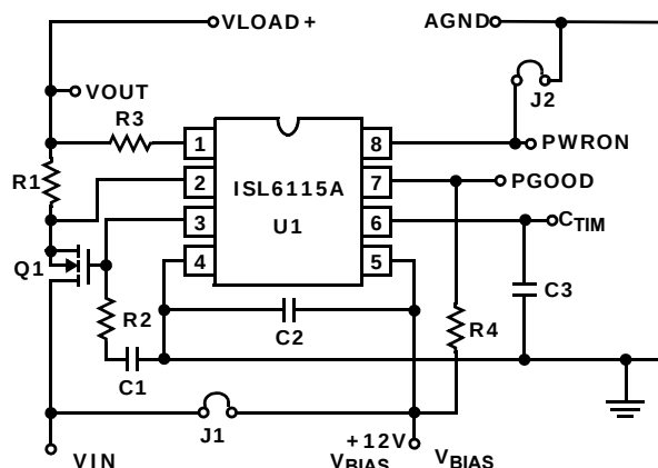
FIGURE 14. ISL6115AEVAL1Z HIGH SIDE SWITCH APPLICATION and PHOTOGRAPH
