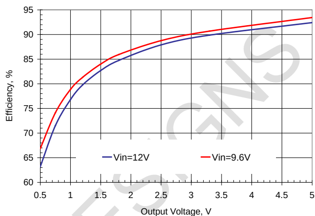
Figure 3. Efficiency vs. Output Voltage, Iout=5A
