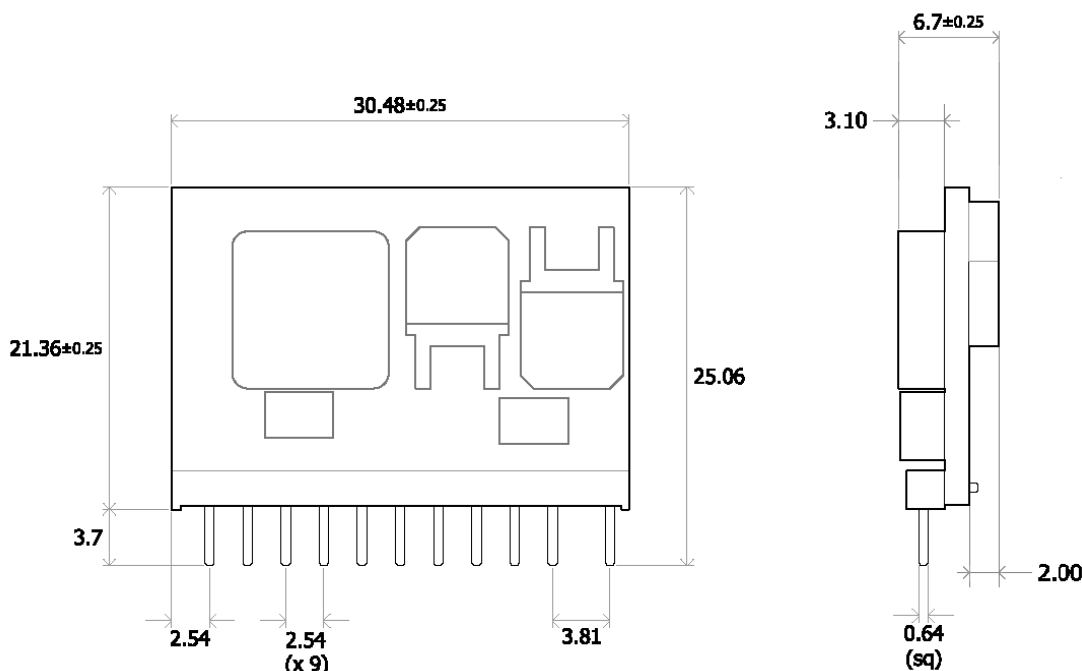
Figure 15. Mechanical Drawing
