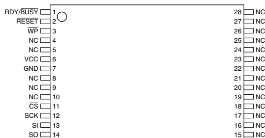
Figure 2-2. CASON – Top View through Package
