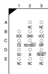
Figure 2-5. CBGA Top View through Package
