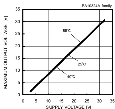
Fig. 28 Maximum Output Voltage - Supply Voltage ( R_L=10[k\Omega] )
