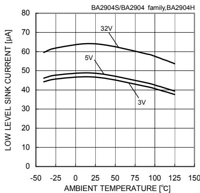
Fig. 59 Low Level Sink Current - Ambient Temperature (VOUT=0.2[V])
