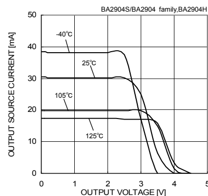
Fig. 54 Output Source Current - Output Voltage (VCC=5[V])
