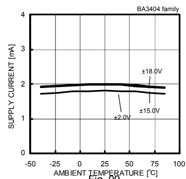
Fig. 99 Supply Current - Ambient Temperature
