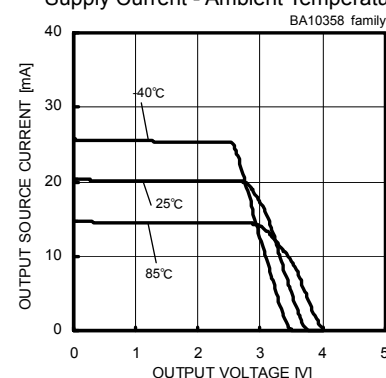
Fig. 6 Output Source Current - Output Voltage ( V_{CC}=5[V] )
