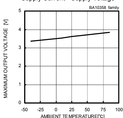
Fig. 5 Maximum Output Voltage - Ambient Temperature ( V_{CC}=5[V] , R_L=2[k\Omega] )
