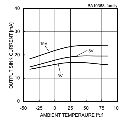
Fig. 9 Output Sink Current - Ambient Temperature ( V_{OUT}=V_{CC} )
