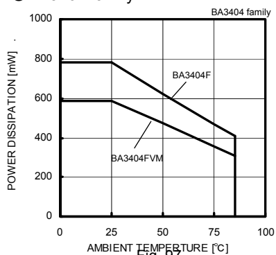
Fig. 97 Derating Curve
