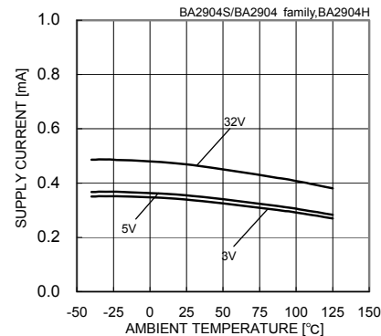
Fig. 51 Supply Current - Ambient Temperature
