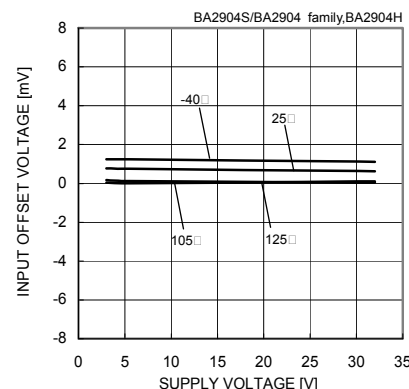
Fig. 60 Input Offset Voltage - Supply Voltage (VICM=0[V], VOUT=1.4[V])
