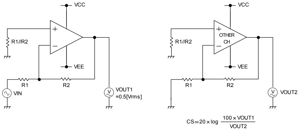
Fig. 123 Measurement Circuit 3
