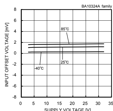
Fig. 36 Input Offset Voltage - Supply Voltage ( V_{cm}=0[V] , V_{OUT}=1.4[V] )
