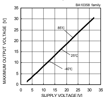
Fig. 4 Maximum Output Voltage - Supply Voltage ( R_L=10[k\Omega] )
