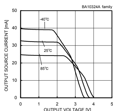
Fig. 30 Output Source Current - Output Voltage ( V_{CC}=5[V] )
