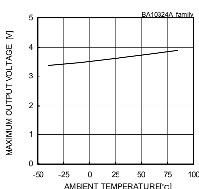
Fig. 29 Maximum Output Voltage - Ambient Temperature ( V_{CC}=5[V] , R_L=2[k\Omega] )
