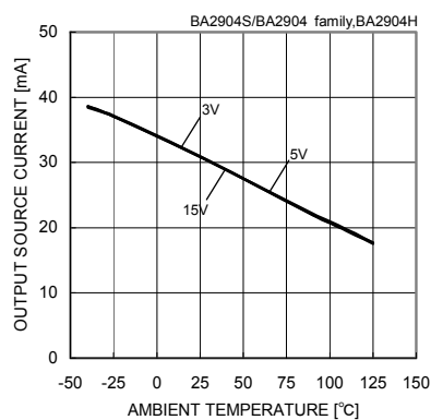
Fig. 55 Output Source Current - Ambient Temperature (VOUT=0[V])
