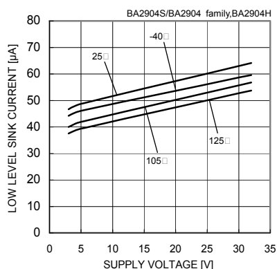
Fig. 58 Low Level Sink Current - Supply Voltage (VOUT=0.2[V])
