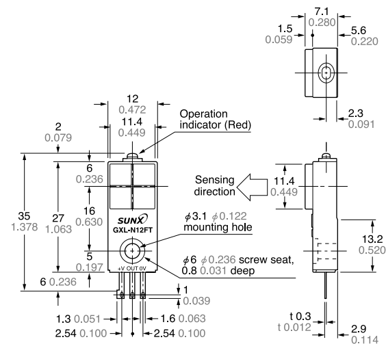
GXL-N12FT type Sensor
