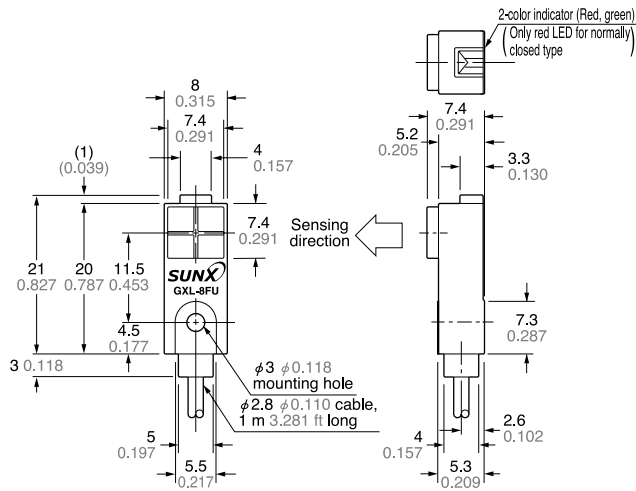
GXL-8FU type Sensor
