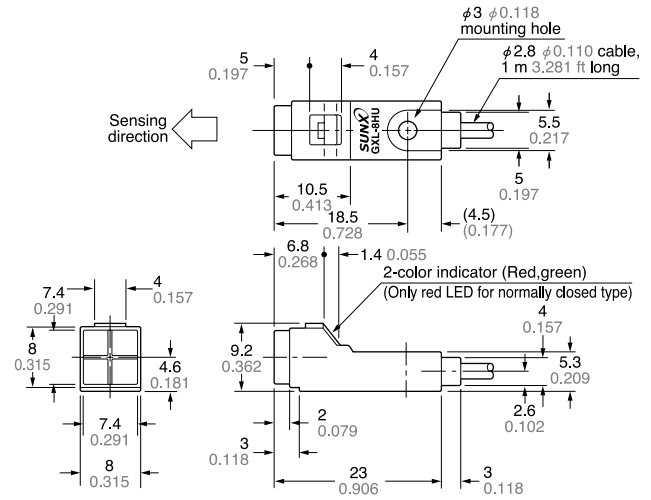
GXL-8HU type Sensor
