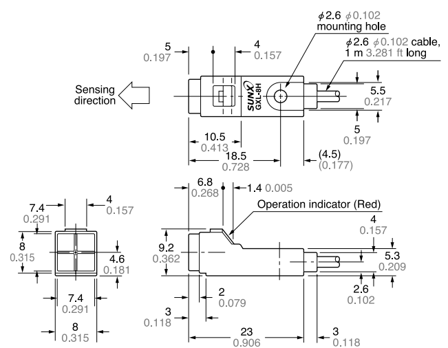
GXL-8H type Sensor
