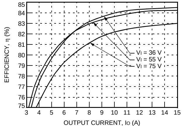
Figure 4. Typical JAW075A Efficiency vs. Output Current at Room Temperature
