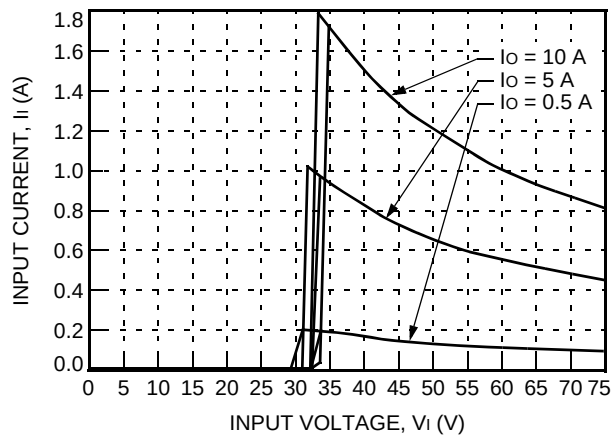
Figure 1. Typical JAW050A Input Characteristics at Room Temperature
