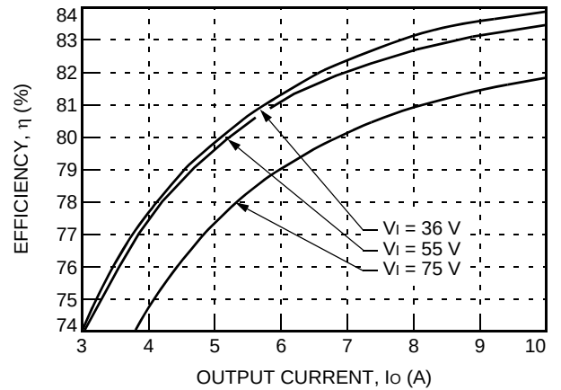
Figure 3. Typical JAW050A Efficiency vs. Output Current at Room Temperature
