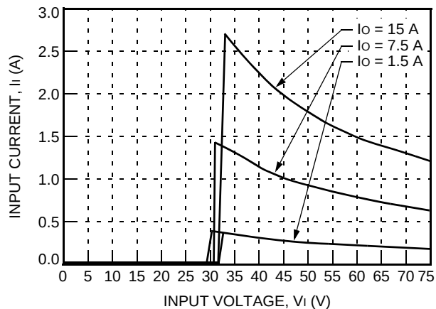
Figure 2. Typical JAW075A Input Characteristics at Room Temperature
