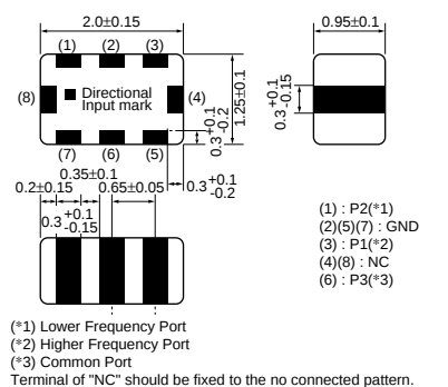
LFD21_DP1 Series
