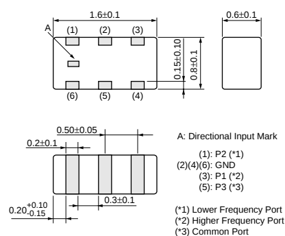
LFD18_DPF Series
