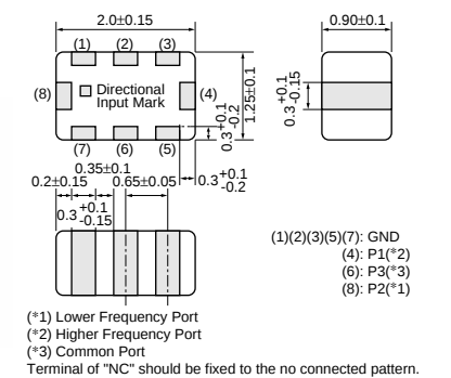
LFD21_DP3 Series
