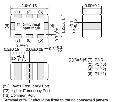
LFD21_DP4 Series
