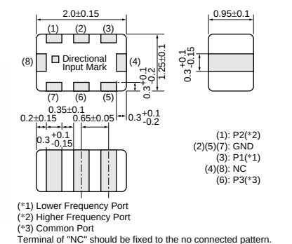
LFD21_DP2 Series
