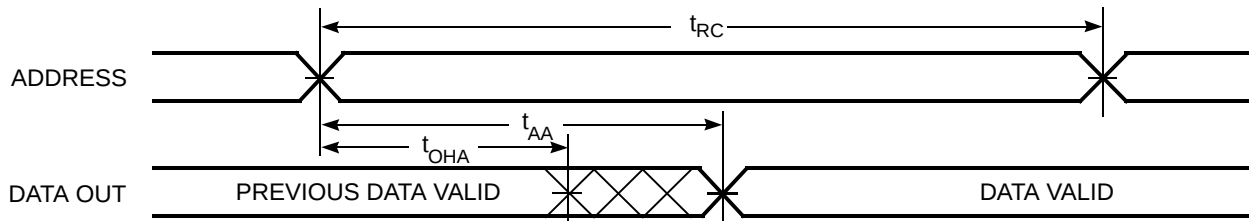
Figure 6. Read Cycle No. 2 ( \overline{\text{OE}} controlled) [17, 18]
