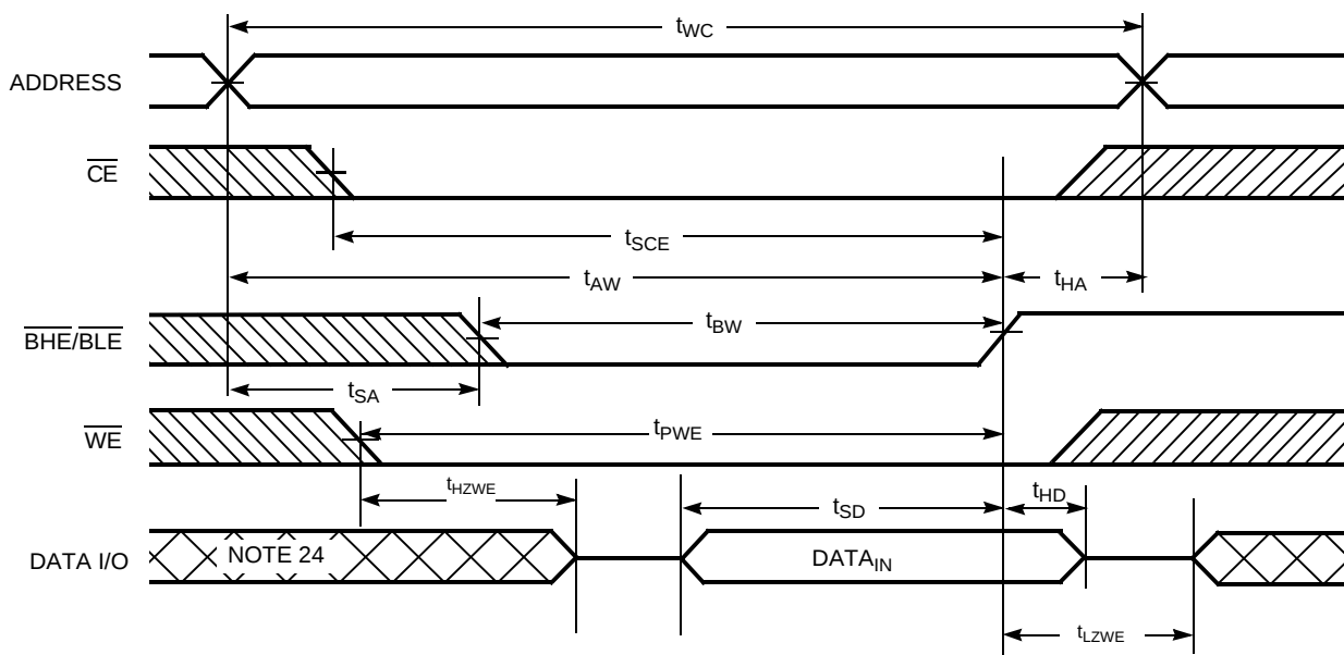
Figure 10. Write Cycle No. 4 ( \overline{\text{BHE/BL}} controlled, \overline{\text{OE}} LOW) [23]
