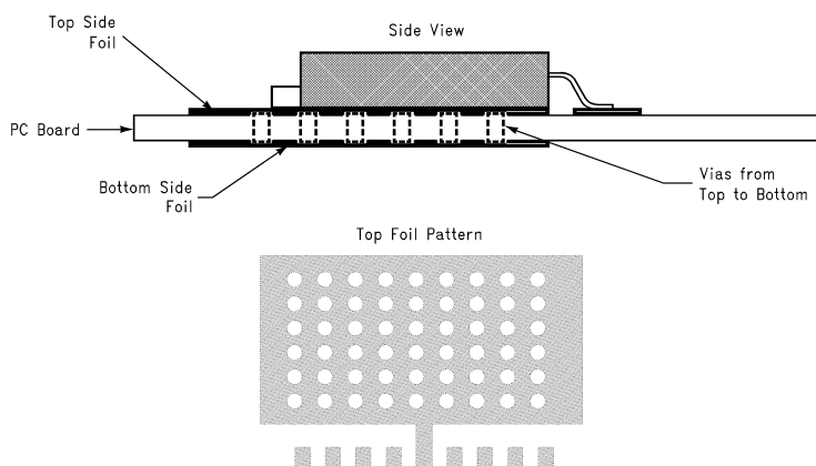
Figure 24. Typical TO-263 PC Board Heatsinking
