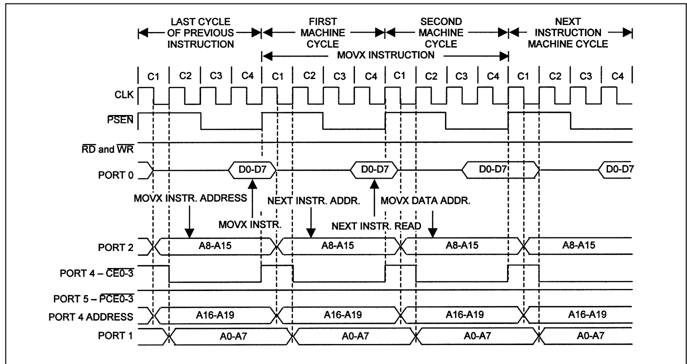
Figure 17. Nonmultiplexed 2-Cycle Data Memory \overline{\text{CE0-3}} Read
