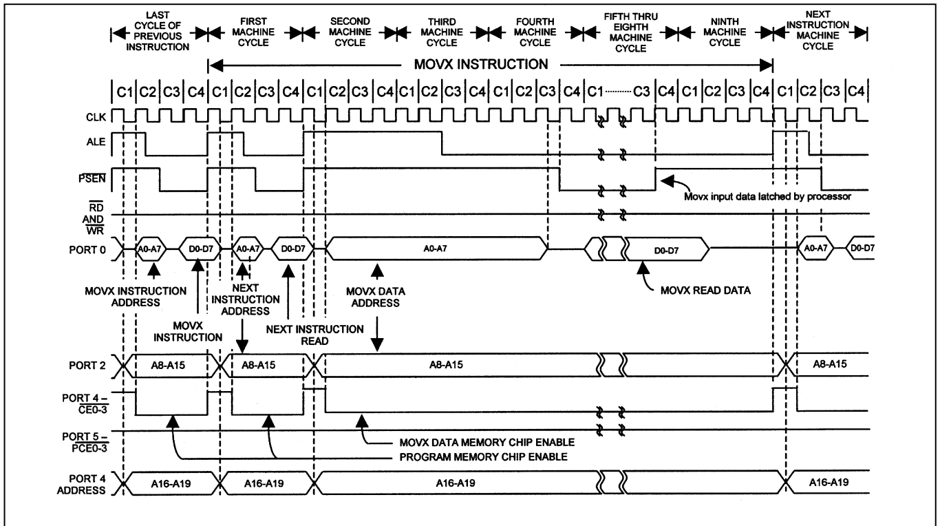
Figure 11. Multiplexed 9-Cycle Data Memory \overline{\text{CE0-3}} Read
