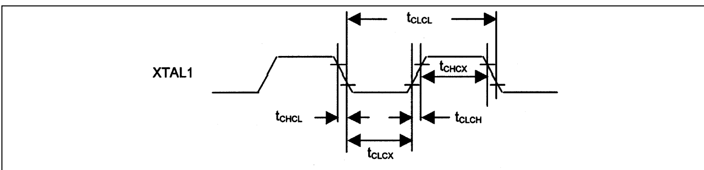
Figure 25. External Clock Drive
