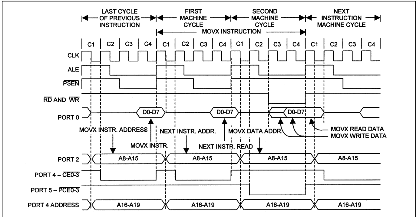
Figure 16. Nonmultiplexed 2-Cycle Data Memory \overline{\text{PCE0-3}} Read or Write
