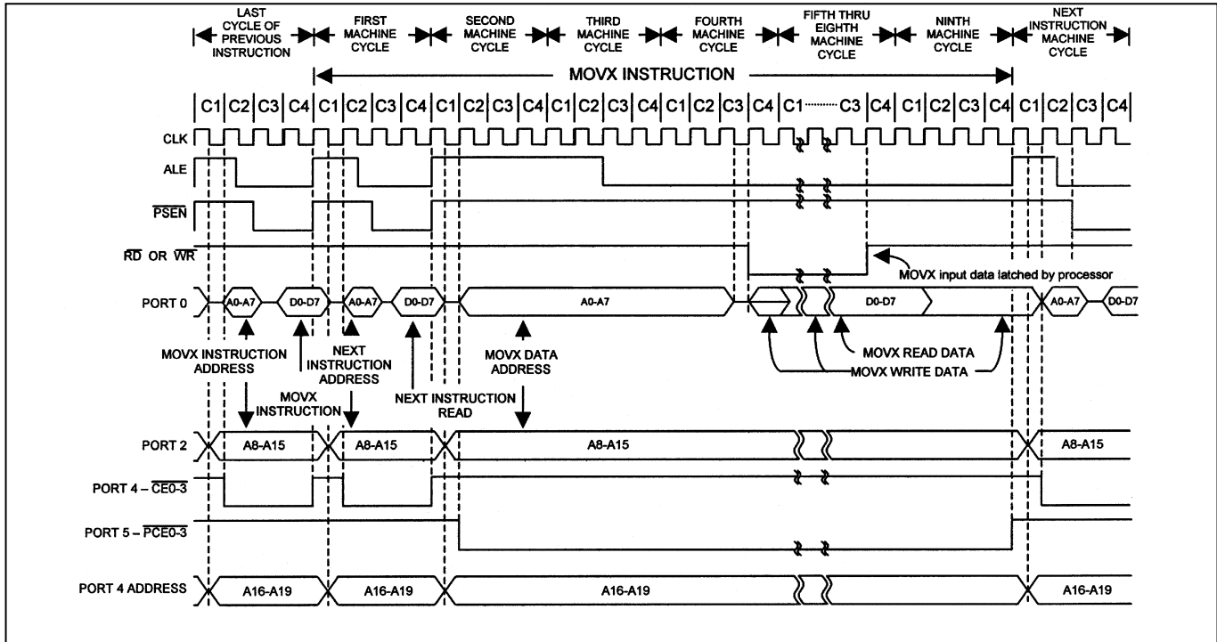
Figure 10. Multiplexed 9-Cycle Data Memory \overline{\text{PCE0-3}} Read or Write
