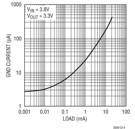
GND Pin Current vs I_{\text{LOAD}}
