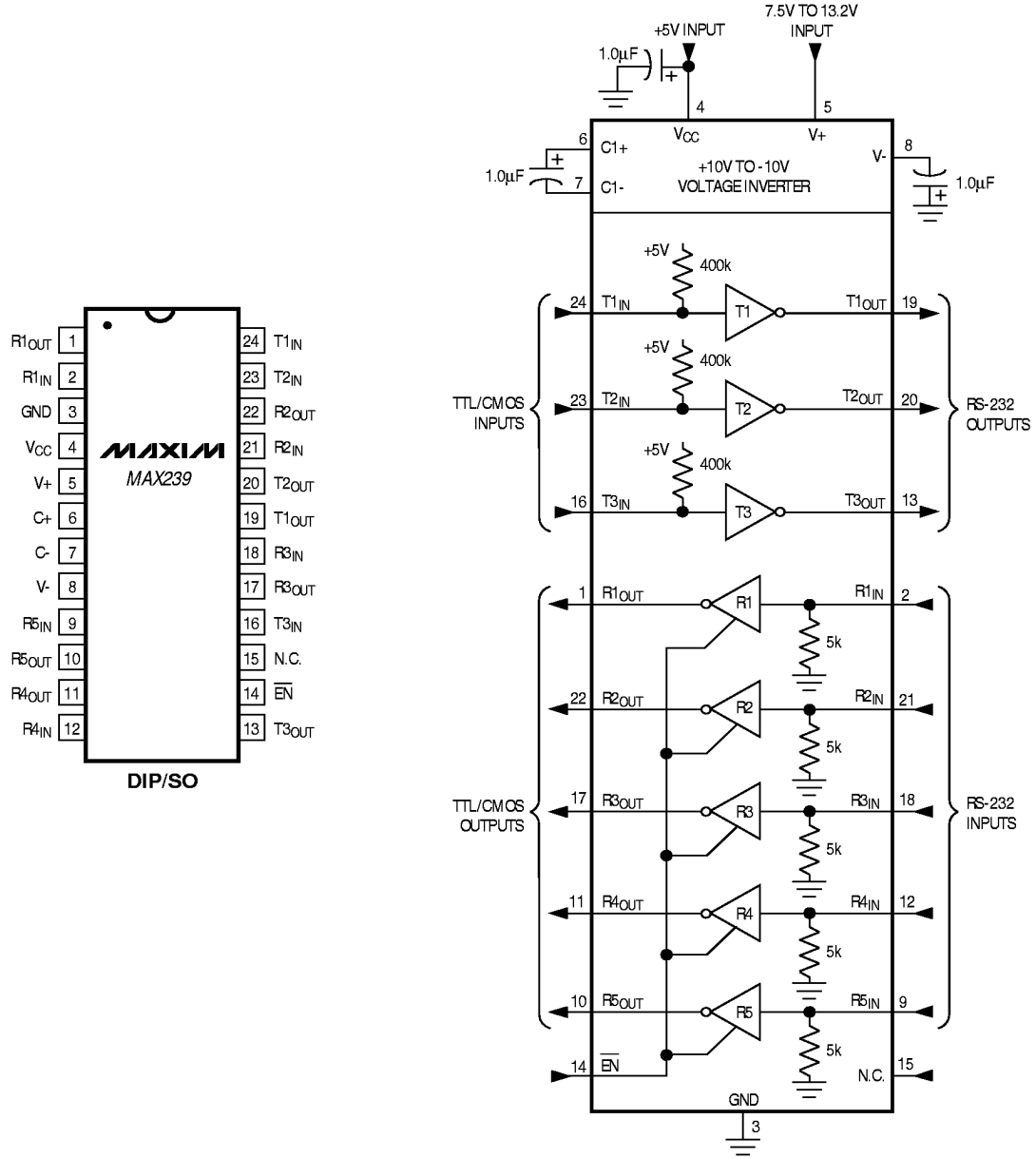
Figure 17. MAX239 Pin Configuration and Typical Operating Circuit
