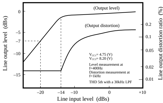
Line AGC input/output characteristics
