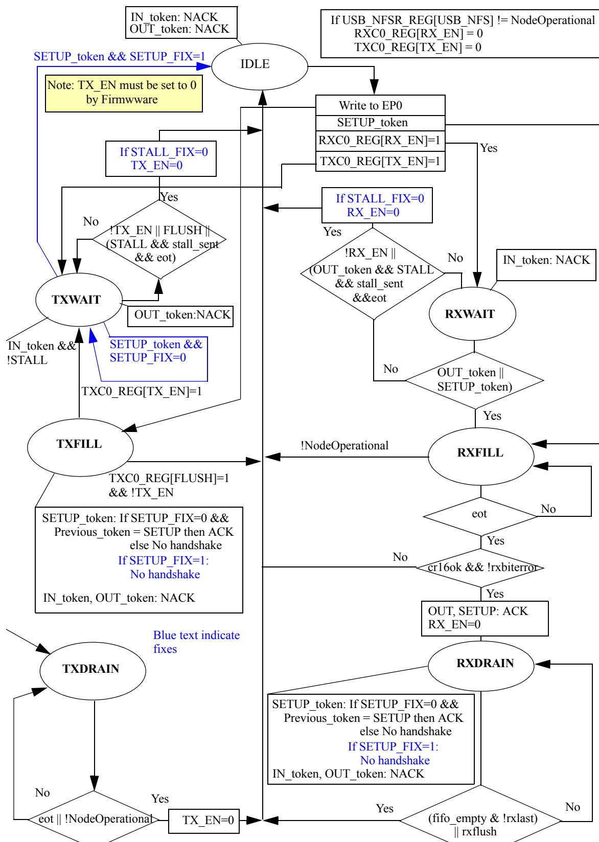
Figure 114: Endpoint 0 Operation
