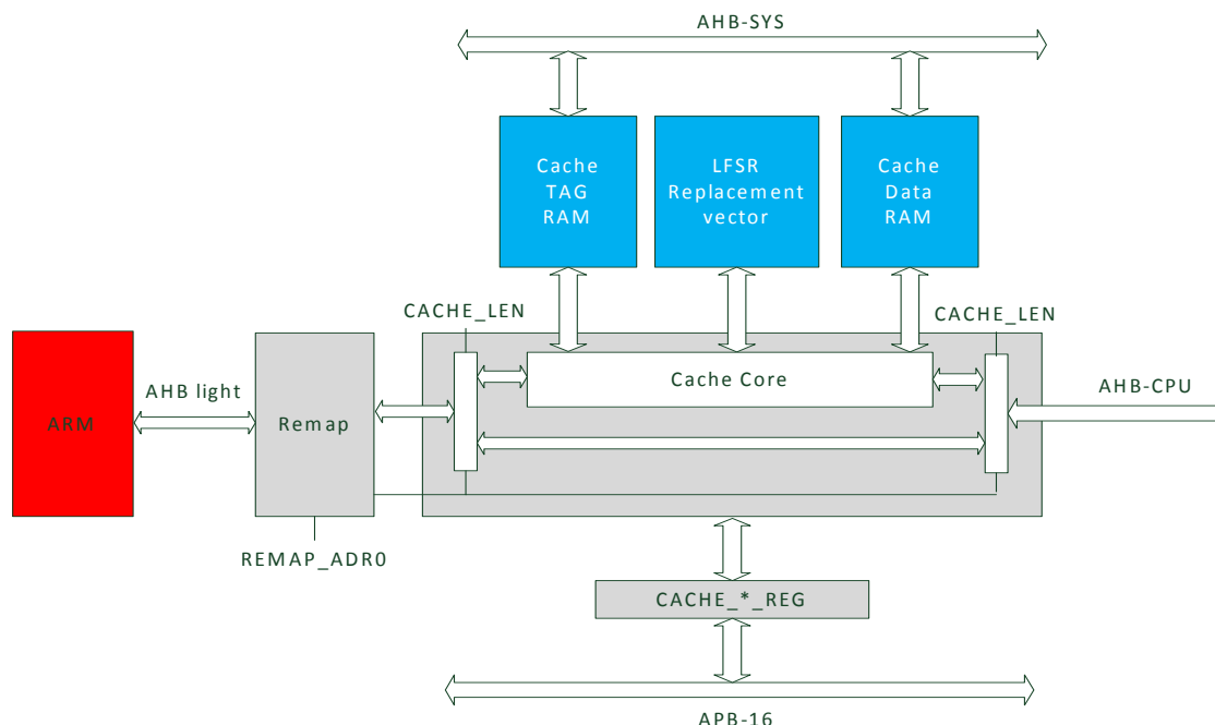
Figure 39: Cache controller block diagram
