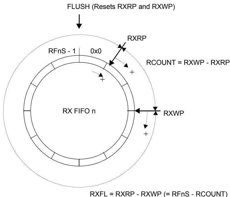
Figure 116: Rx FIFO operation
