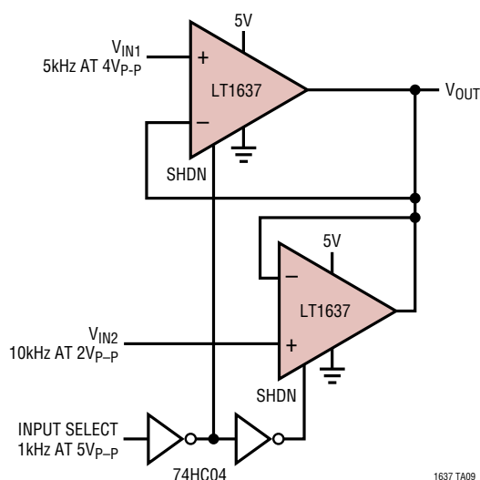
MUX Amplifier
