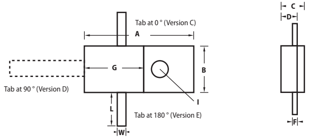
Style 1 Two Hole Flanged Model
