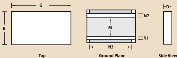
Style 4 Surface Mount Chip for PCB
