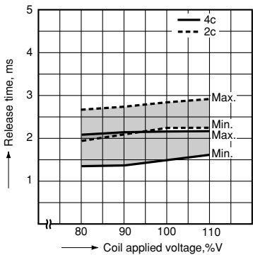
4. Release time for single side stable
