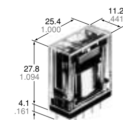
2C Vertical type (PC board)
