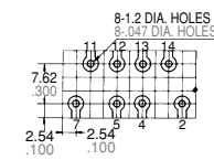
PC board pattern (Copper-side view)
