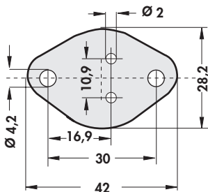
TO 3/4
