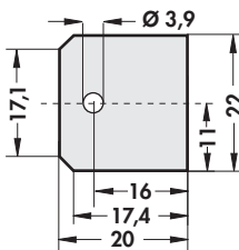
TO 218 Multiwatt
