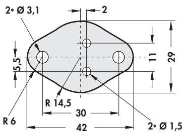
TO 3
