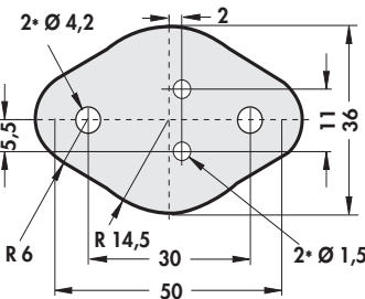
TO 3 M
