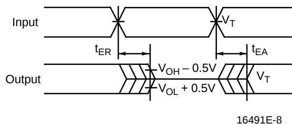
d. Input to output disable/enable
