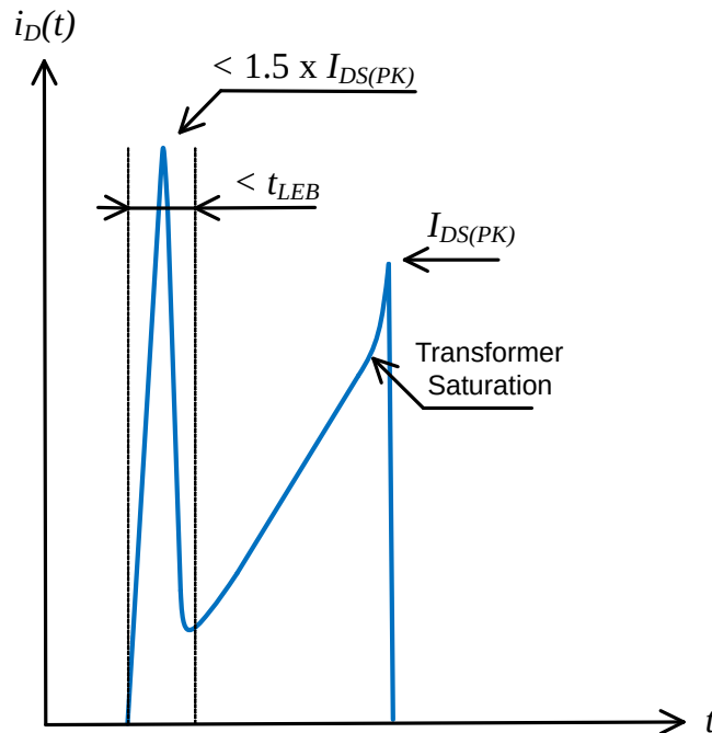
Figure 4. Spike Limits
