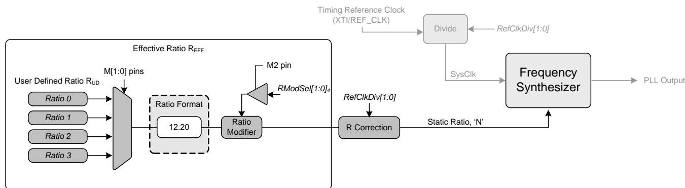
Figure 6. Ratio Feature Summary
