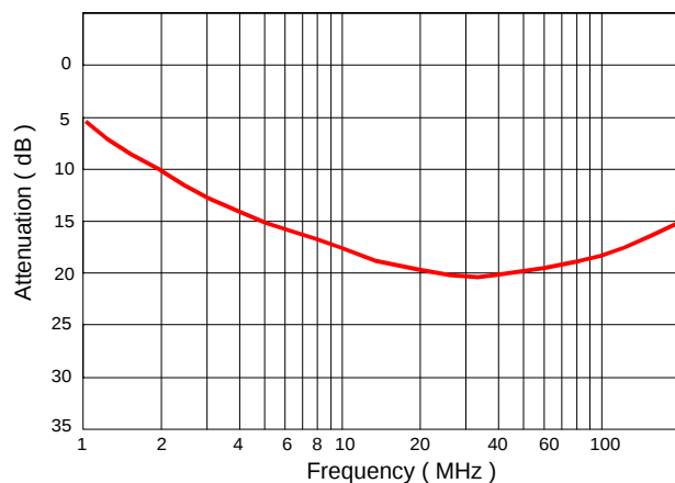
TYPICAL ATTENUATION
