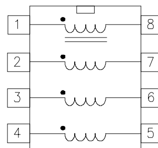
SCHEMATIC DIAGRAM Top View
