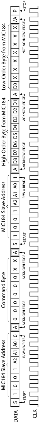
Figure 4. READ_WORD Protocol
