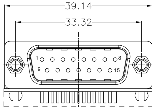
MALE 15P CONTACT D-SUB CONNECTOR
