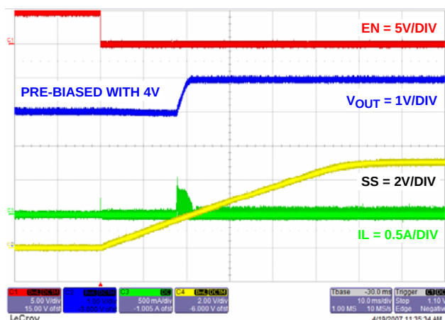
FIGURE 23. SOFT-START WITH PRE-BIASED
