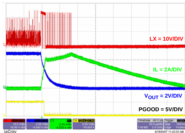
FIGURE 25. OUTPUT SHORT CIRCUIT
