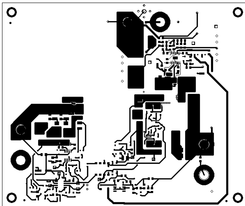
Figure 19. Top Route
