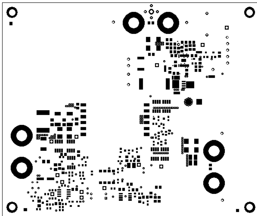
Figure 18. Top Mask
