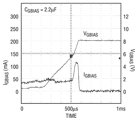
G_{BIAS} vs I_{GBIAS} (Charging 2.2 \mu F)
