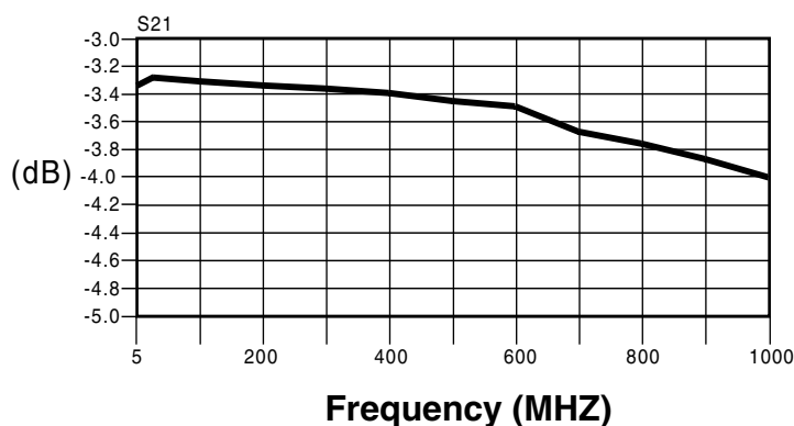
INSERTION LOSS
