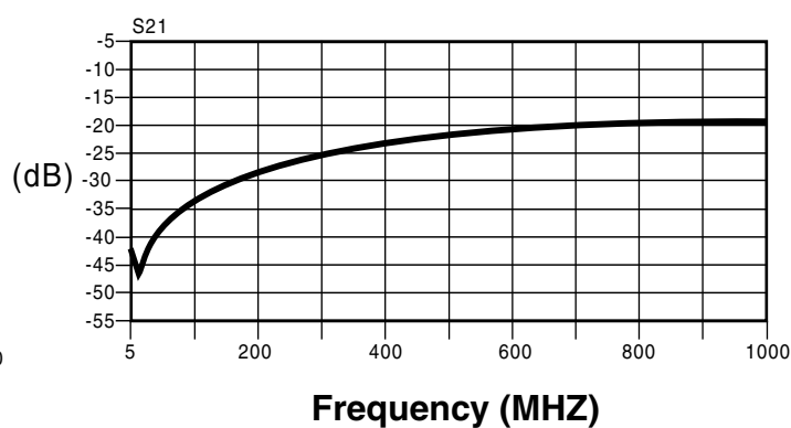
ISOLATION
