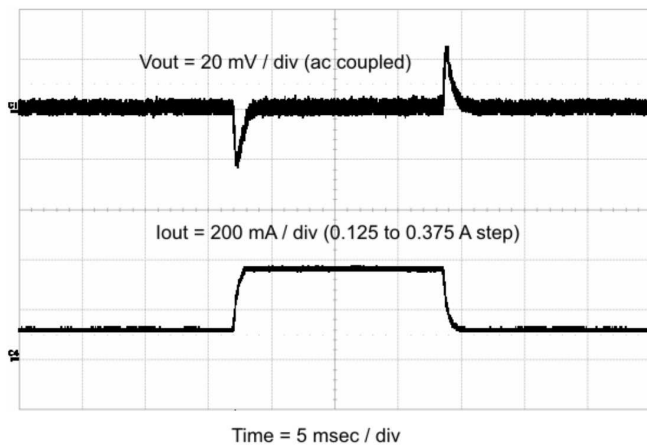
Figure 52. Load Transient
