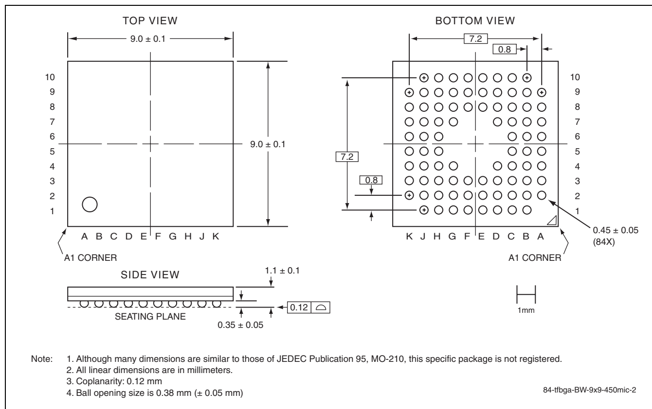
FIGURE 13-1: 84-ball Thin, Fine-pitch, Ball Grid Array (TFBGA) SST Package Code: BW
