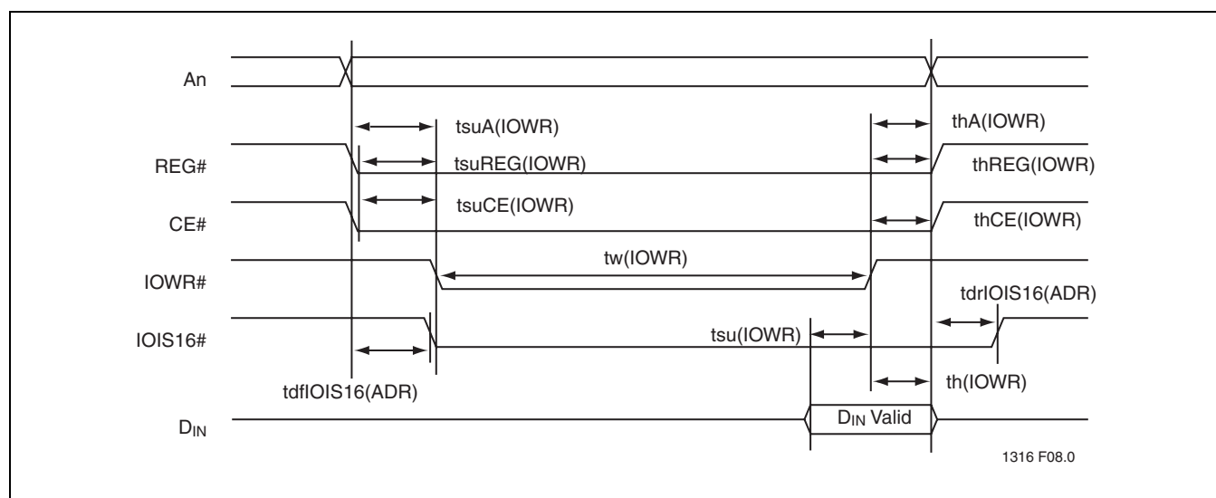
FIGURE 10-7: I/O Write Timing Diagram
