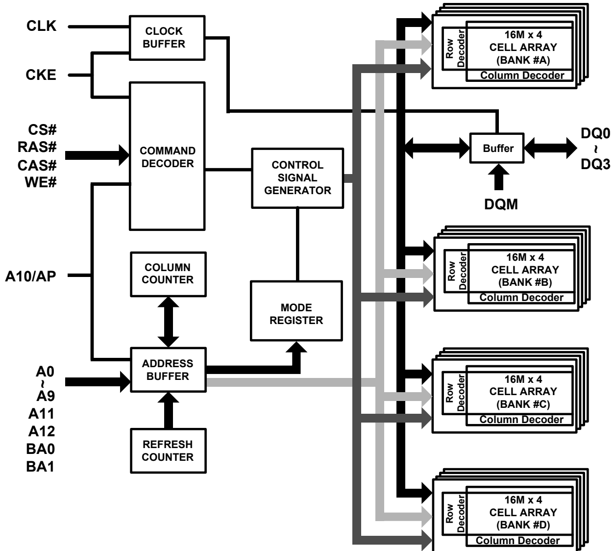
Figure 2. Block Diagram
