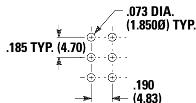
PC Mounting
