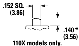
S2 0.140" High
