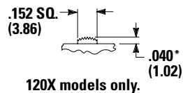
S1 0.040" High
