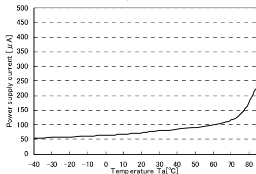
I_{CCR} timer mode(sub oscillation) temperature characteristics Vcc:5.5V, LVD is Off
