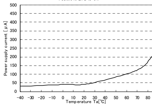
I_{CCR} stop mode (sub oscillation) temperature characteristics Vcc:5.5V, LVD is Off
