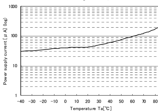
I_{CCR} stop mode (sub oscillation) temperature characteristics(semi-log) Vcc:5.5V, LVD is Off
