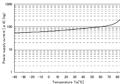
I_{CCR} timer mode(sub oscillation) temperature characteristics(semi-log) Vcc:5.5V, LVD is Off
