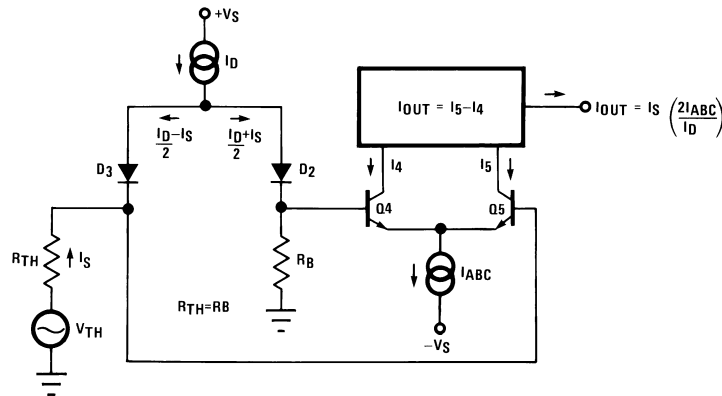
Figure 20. Voltage-Controlled Amplifier
