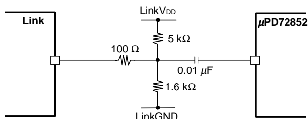
(c) LPS Isolation Barrier Circuit
