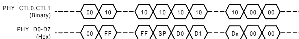
Figure 4-8. Receive Timing
