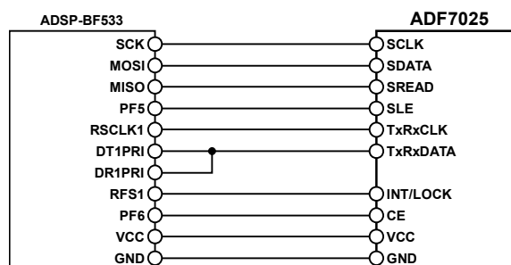
Figure 35. ADSP-BF533 to ADF7025 Connection Diagram
