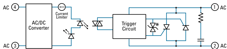
AC control
