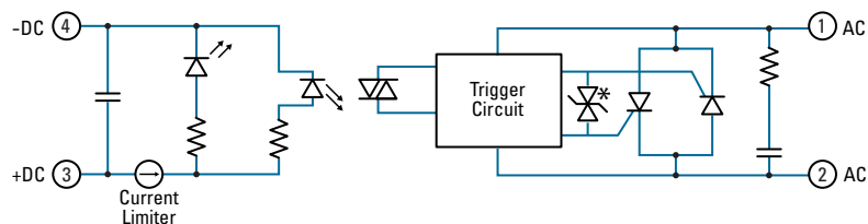
DC control
