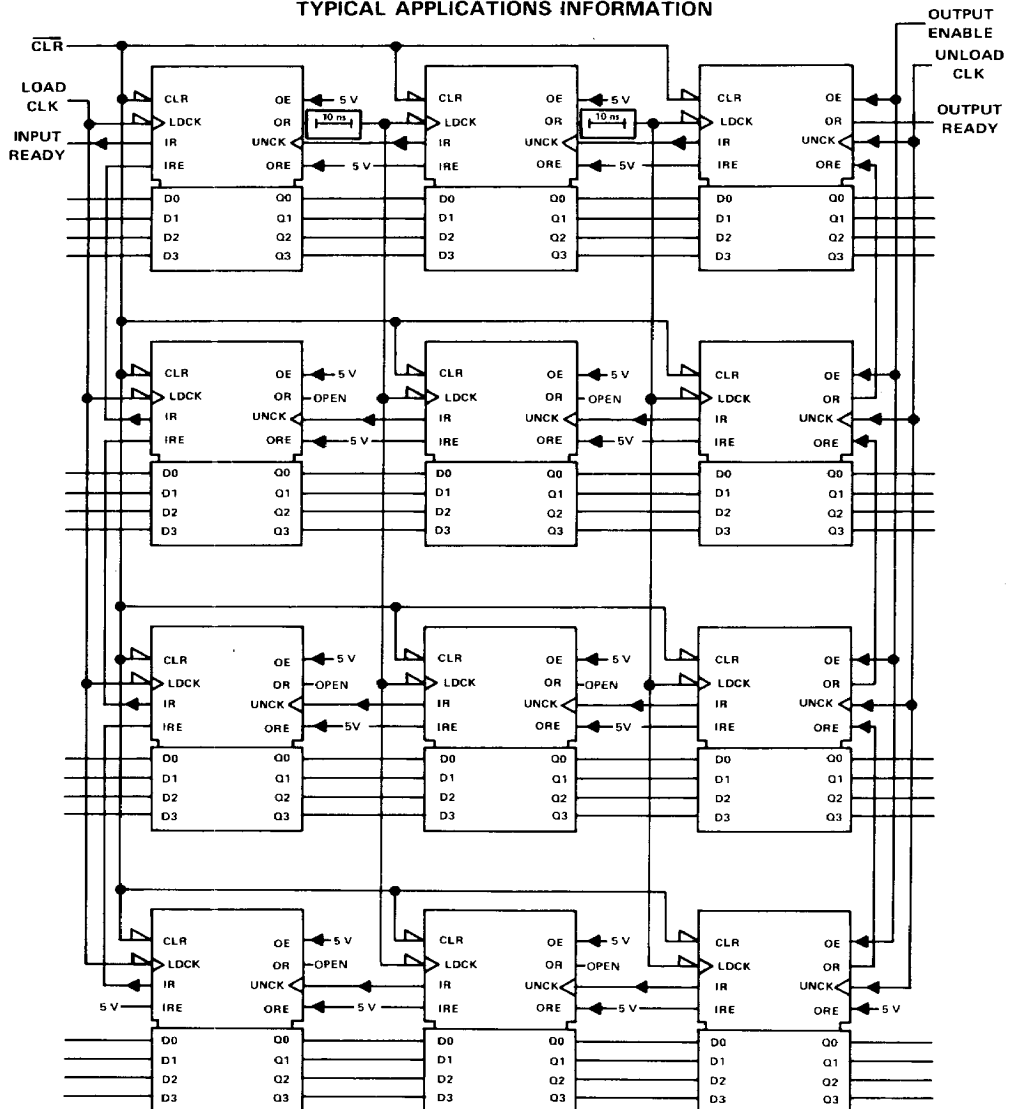
FIGURE 1. 46-WORD BY 16-BIT EXPANSION USING 'LS222
