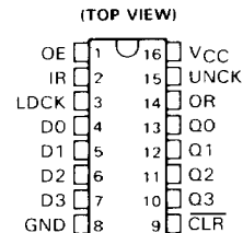
SN54LS224, SN54LS228 . . . J PACKAGE SN74LS224, SN74LS228 . . . J OR N PACKAGE
