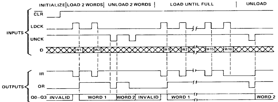
timing diagram
