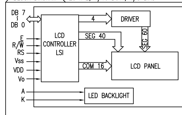
BLOCK DIAGRAM A 20 x 2, 1/16 DUTY, 1/5 BIAS
