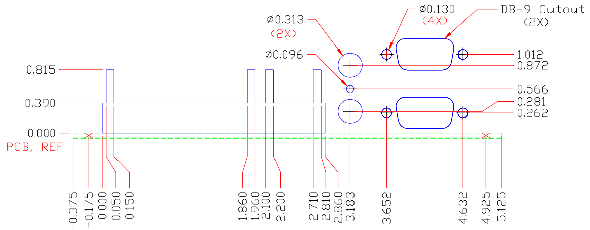
Figure 7. CBL/CBR-8004 Dimensions and Mounting
