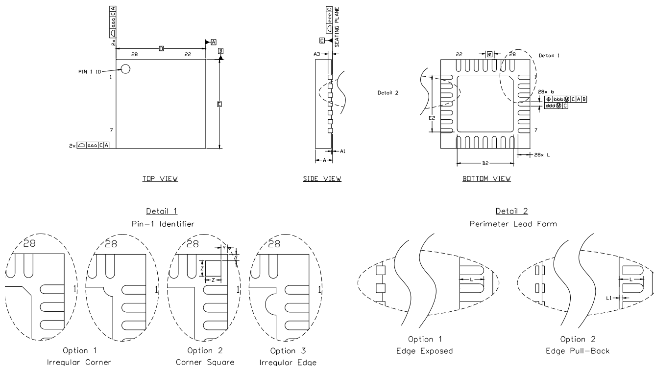
Figure 6. QFN-28 Package Drawing
